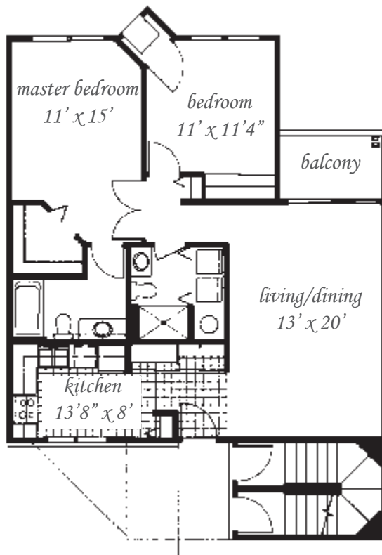
two bedroom two bath 2a, 2b
